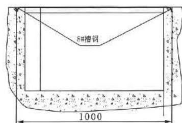
电缆沟深根据电缆弯曲半径确定 The depth of the cable trench is determined according to the cable bending radius;
