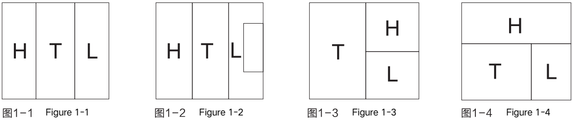
图1 YBM、YBP（ZBW）系列预装式变电站平面布置形式图（H-高压室 T-变压器室 L-低压室） Figure 1 The layout of the YBM, YBP (ZBW) series of prefabricated substations (H-high voltage room, T-transformer room, L-low voltage room)
