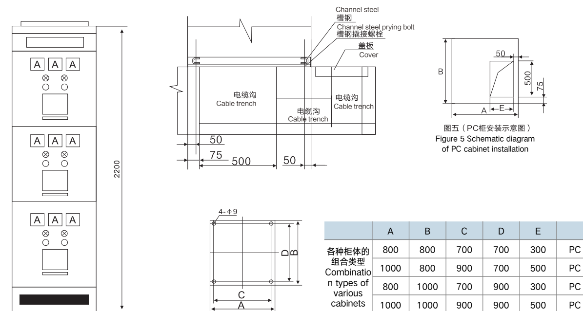
图5 PC柜安装示意图 Figure 5 Schematic diagram of PC cabinet installation
