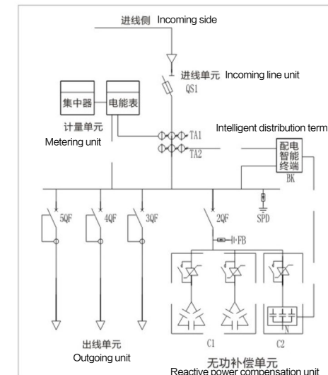
Electrical diagram of 400kVA low-voltage integrated distribution box (I)
