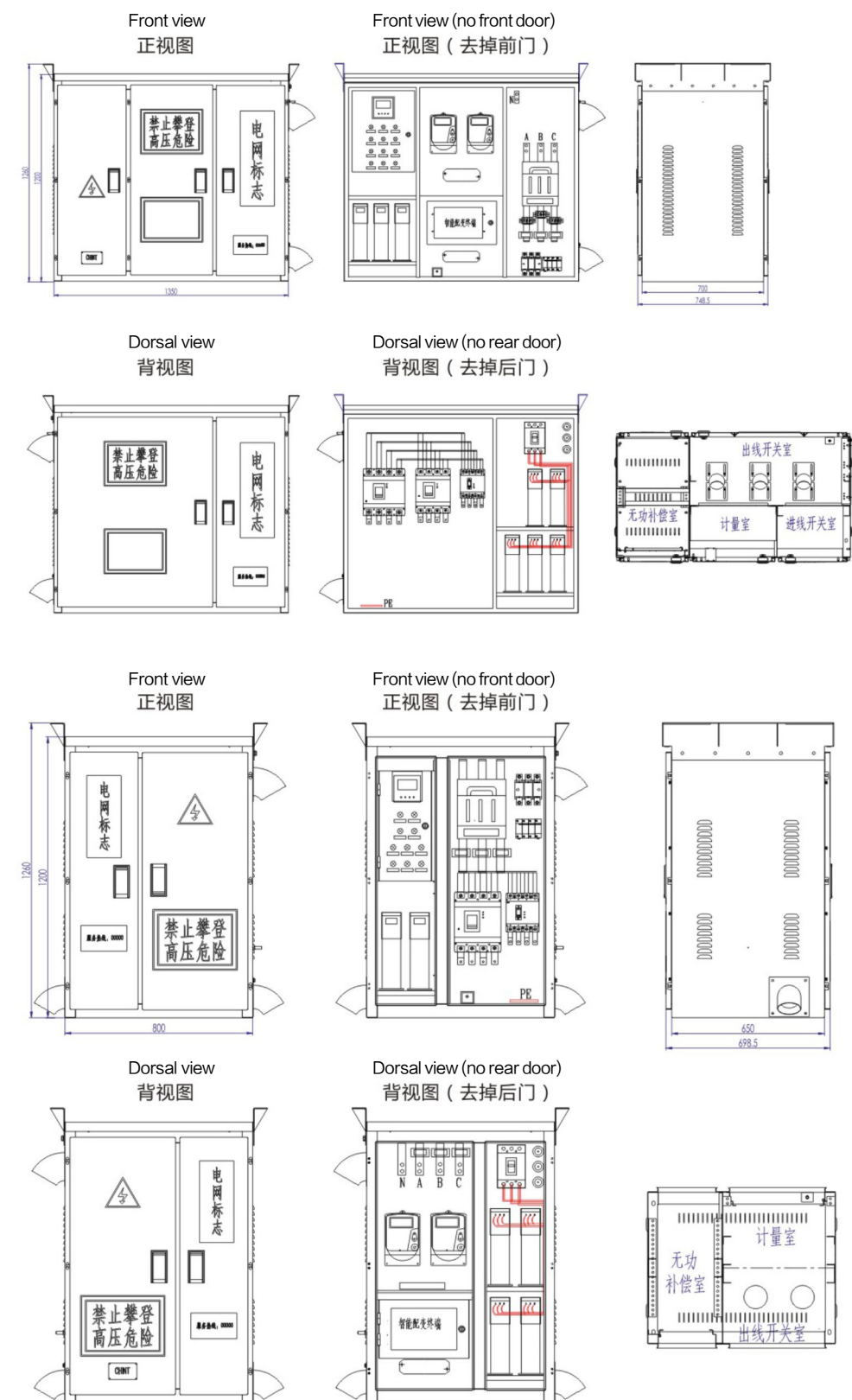
8.3柜内元件布局 Layout of components in the cabinet
