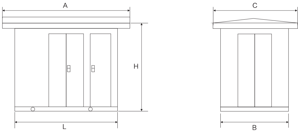
图2 YBM、YBP（ZBW）系列预装式变电站外形图（“目”字型排列） Figure 2 Outline drawing of YBM, YBP (ZBW) series of prefabricated substations (arranged in "目" font)
